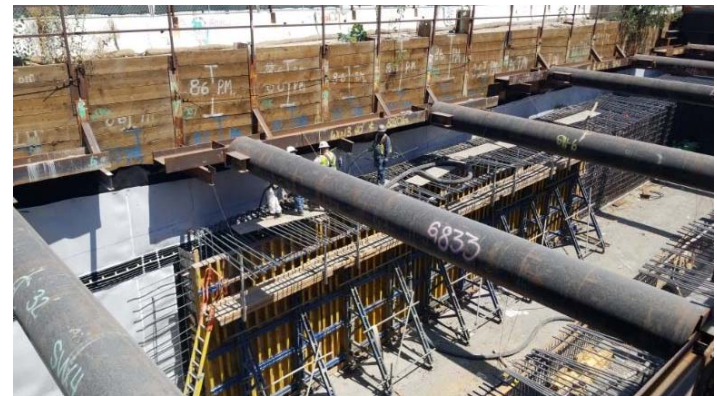
1st Street Cut/Cover Walls pour preparation
