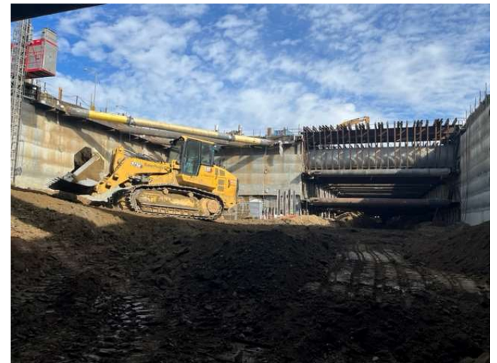
Westwood/VA Hospital Station: Excavation for Level 4 Support
